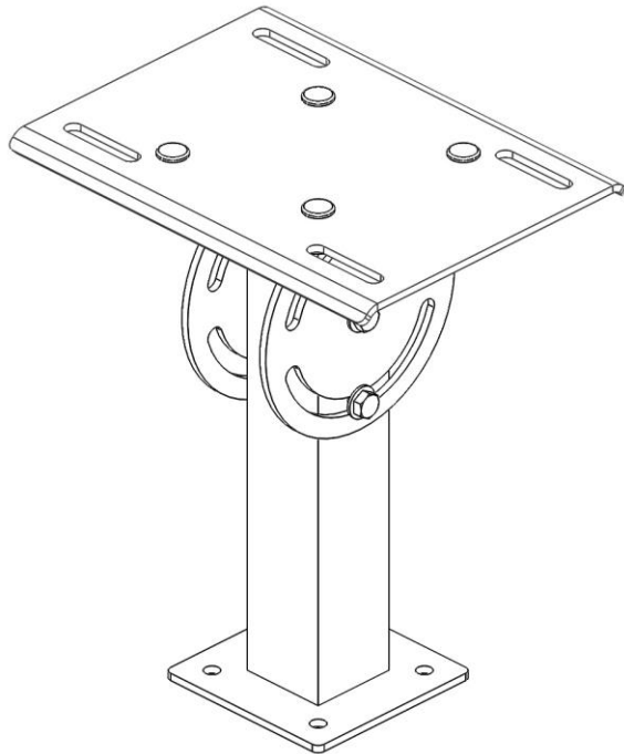
Rigid Mount
